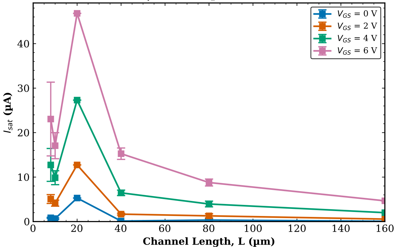
TFT1 Combined (Tr. 1 & 2) I_{sat} vs L | W = 50 \mu\text{m} (mean \pm std)
